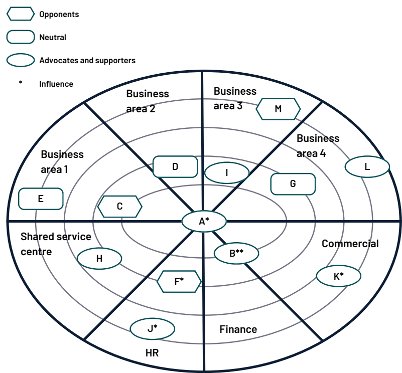
Figure 26.3 Stakeholder landscape
